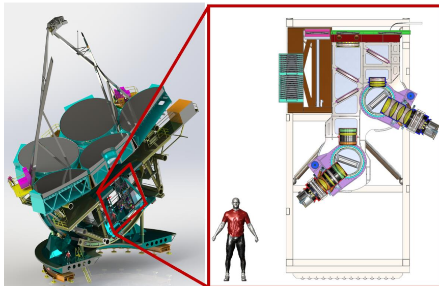
Figure 1. Location of the GMACS instrument within GMT.
