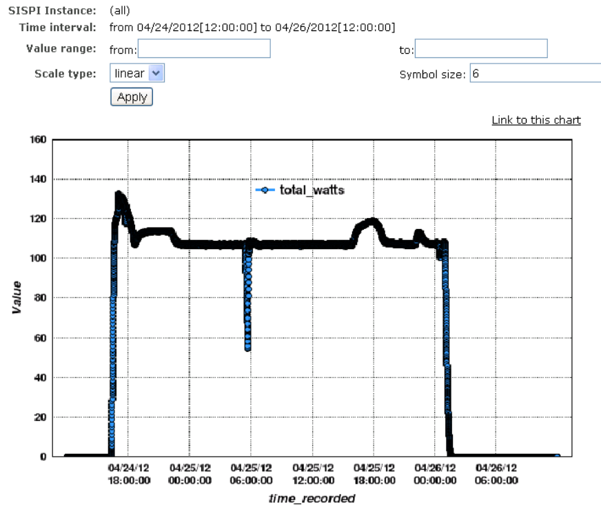
Figure 7. Power (Watts) applied to the focal plate trim heaters, as a function of calendar time, required to maintain -100^{\circ}\text{C} at the focal plate.
