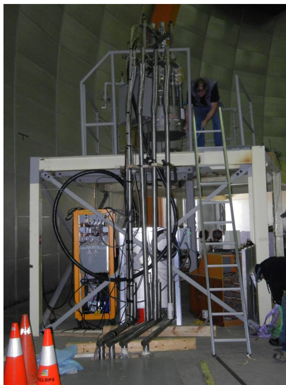
Figure 3. LN2 process station mounted to top of old console room roof. In the old console area is the slow controls rack. LN2 transfer lines are routed from the LN2 process station to the Coudé room and to the Telescope.
