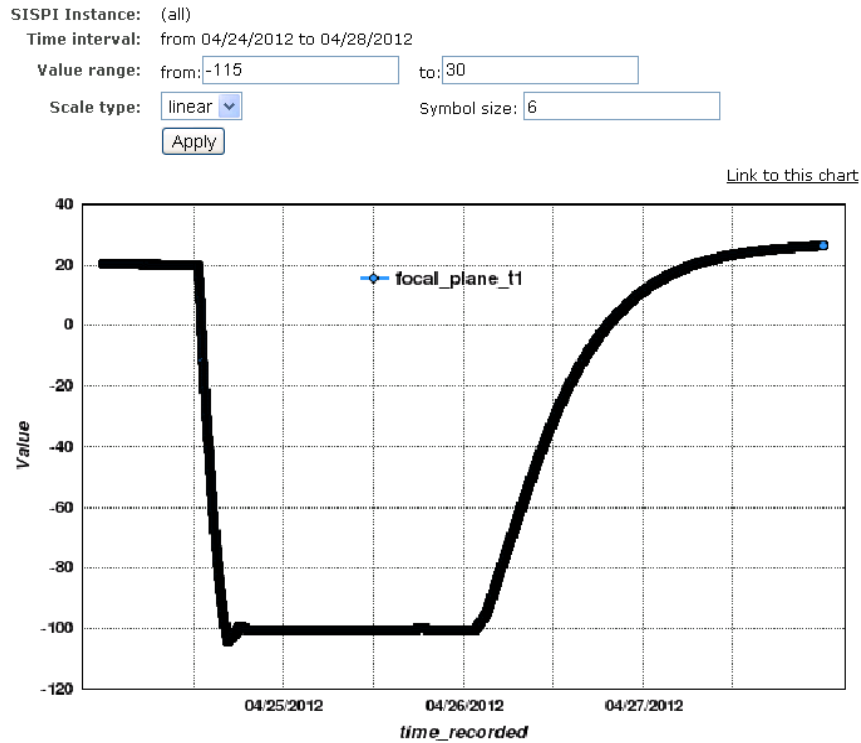
Figure 6. Temperature ( ^{\circ}\text{C} ) at the front of the imager focal plate, as a function of calendar time for the cool down.
