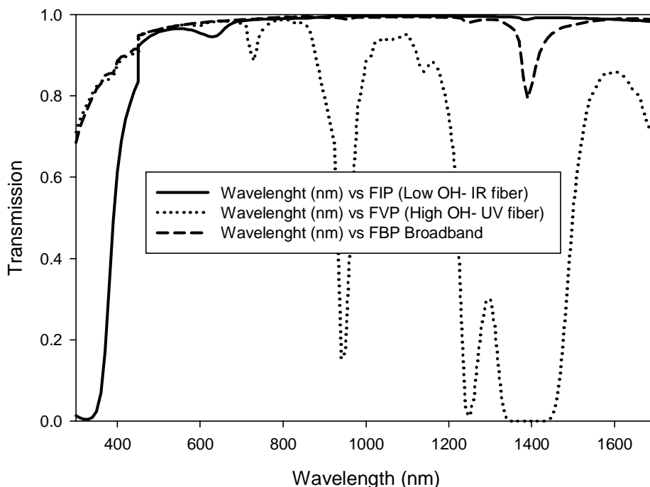
Figure 2. Internal transmission over 10 meter for different fiber types.
