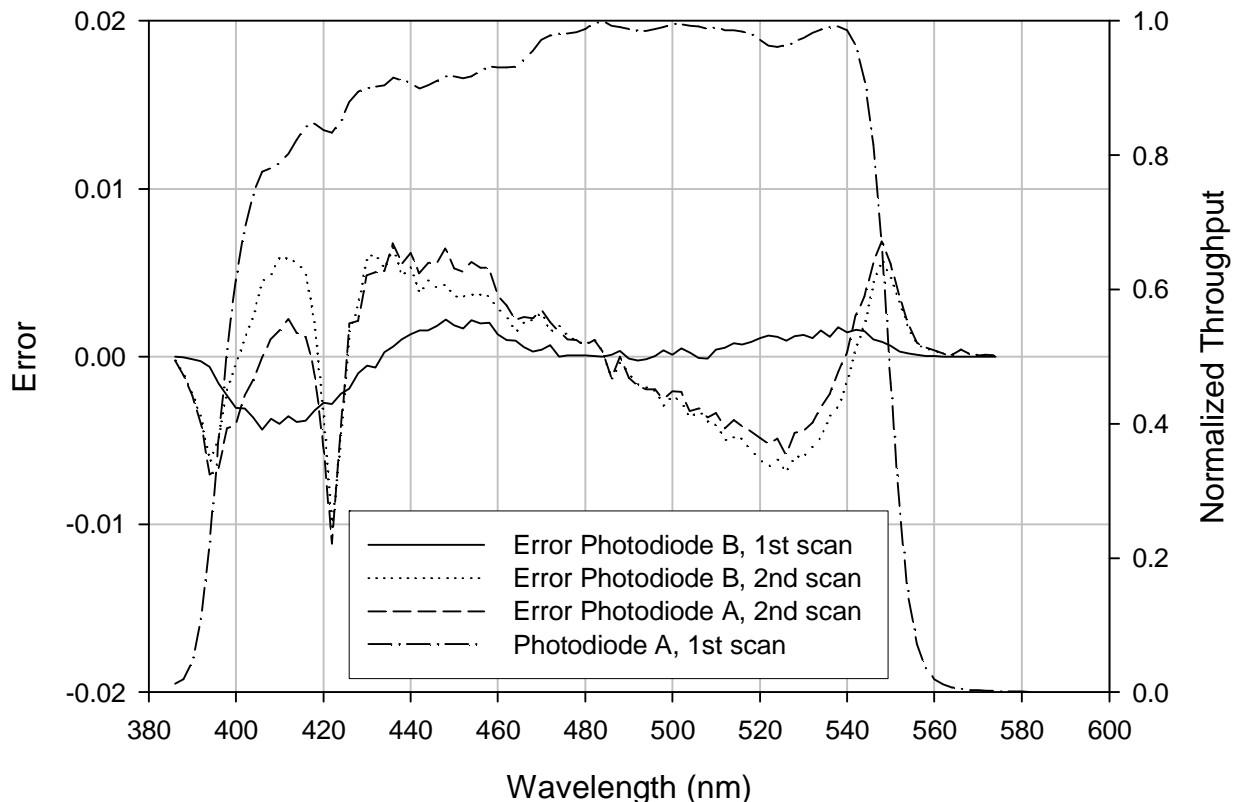
Figure 7. Repeatability of the g filter throughput for 2 separate scans. Error compared to Photodiode A and 1st scan
