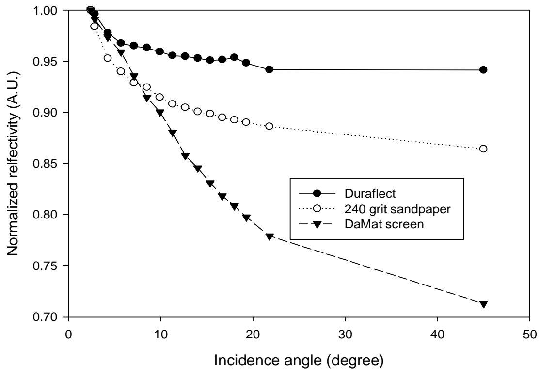
Figure 4. Normalized reflectivity at normal exit angle vs incident angle. Details of the various results are given in the text.
