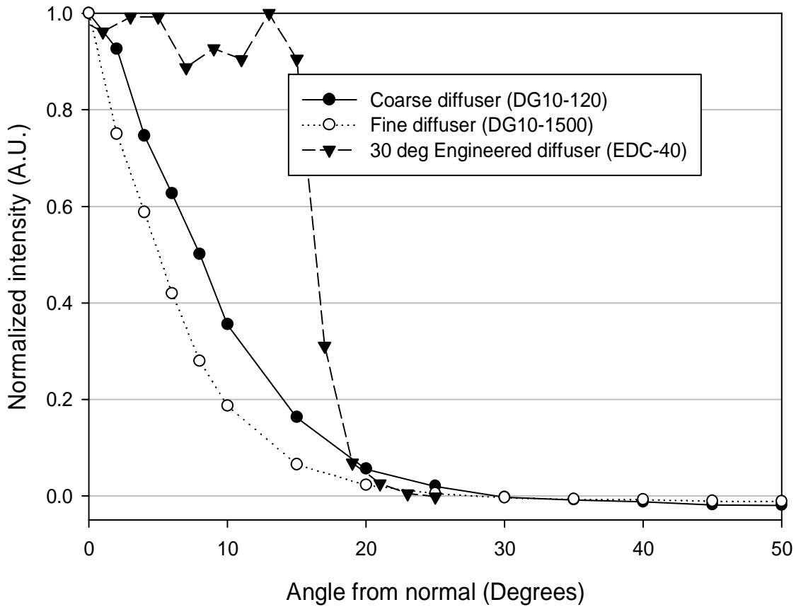
Figure 3. This figure shows the measured far field radial profile of a collimated HeNe laser 1 meter after transmission through 3 different diffusers. The two curves with the filled and empty circles represent the transmission through regular ground glass diffusers from Thorlabs. The triangles represent the transmission through the engineered diffuser from RPC photonics.
