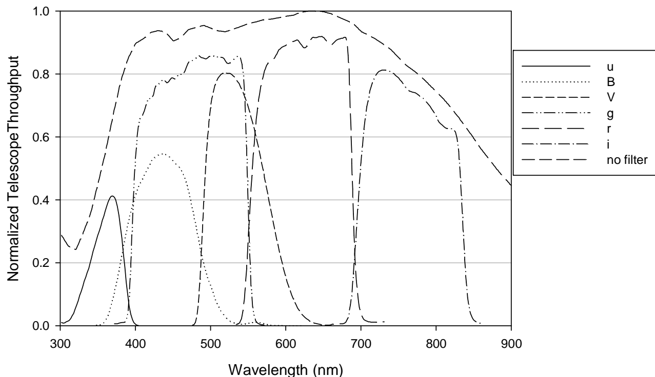
Figure 6. Swope Telescope Throughput
