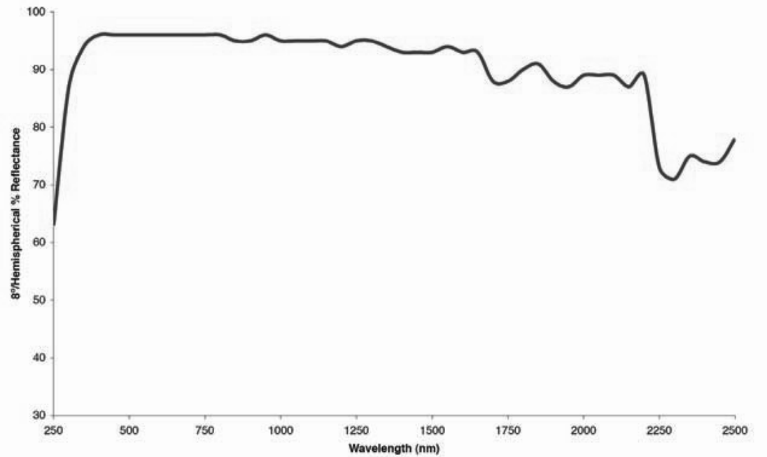
Figure 5. Durafluct reflectivity vs wavelength
