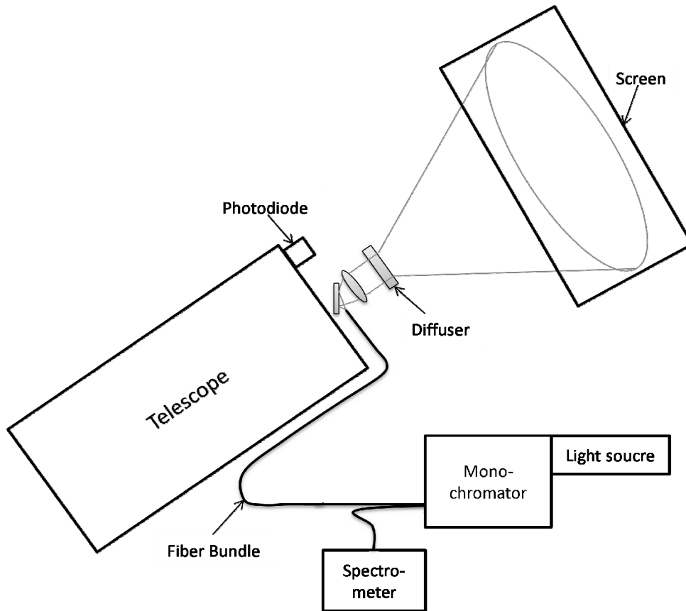
Figure 1. Experimental setup
