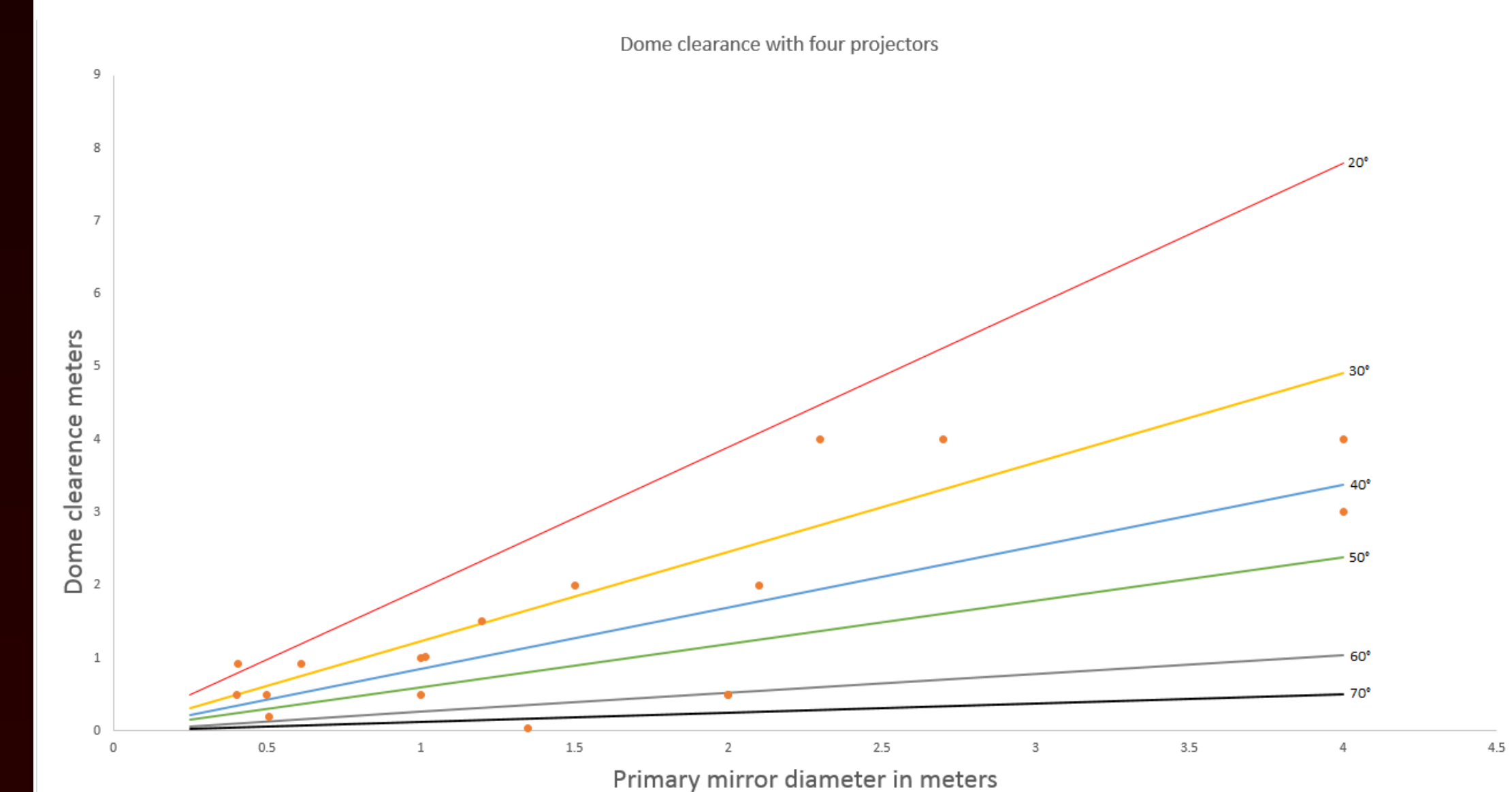
Figure 5: Dome clearance and diffuser angles for four projectors
