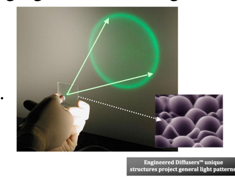
Figure 2: Projection cone[3]
