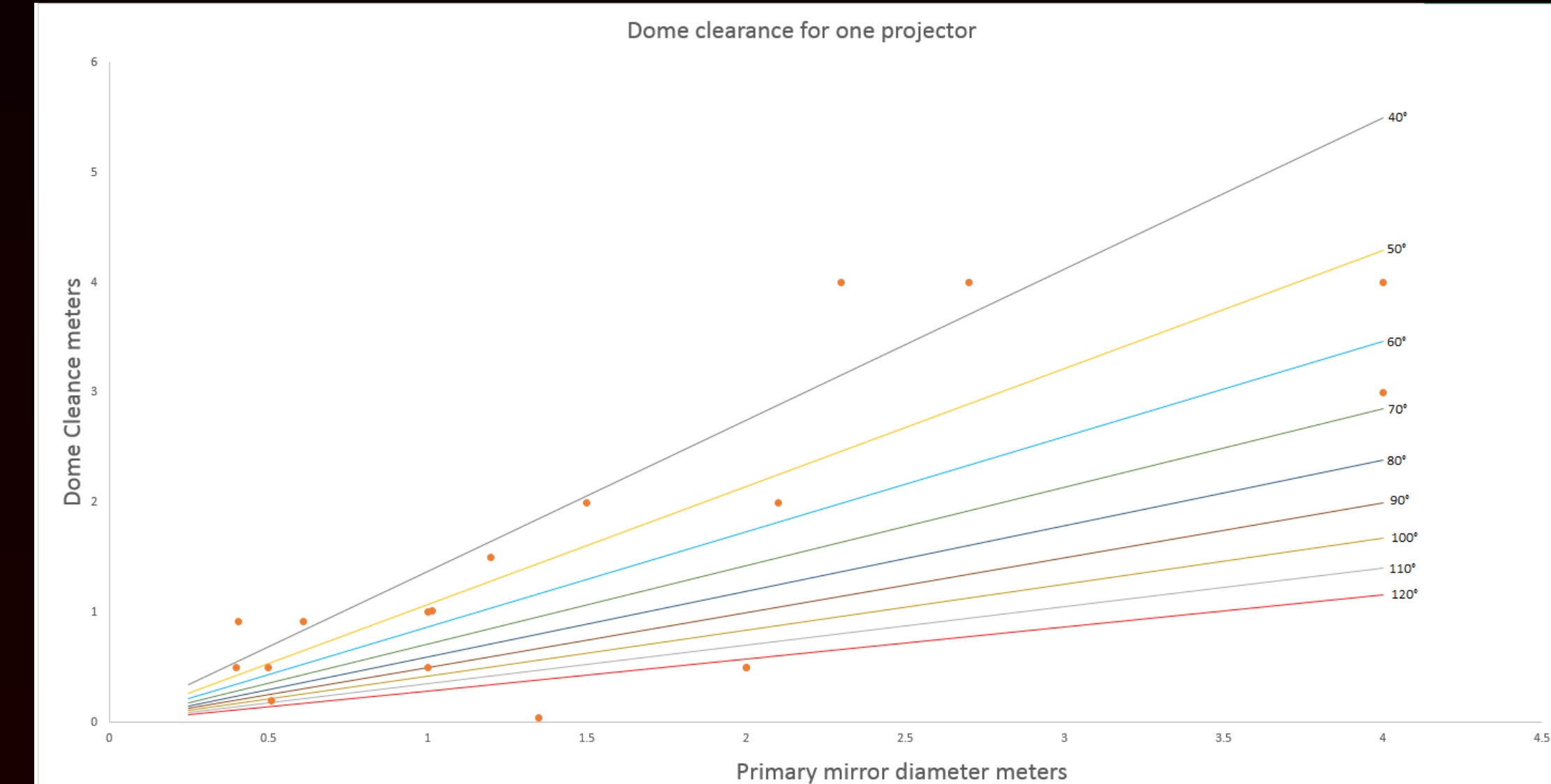
Figure 4: Dome clearance and diffuser angles for one projector
